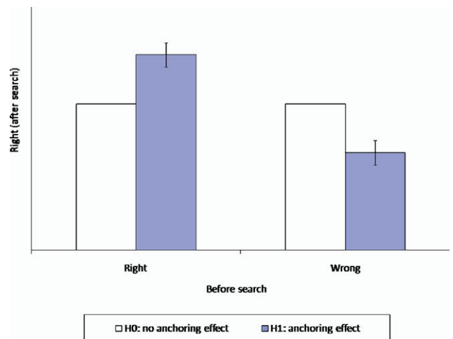
Figure 1. Anchoring effect: the null hypothesis (H0) and the alternative hypothesis (H1).
