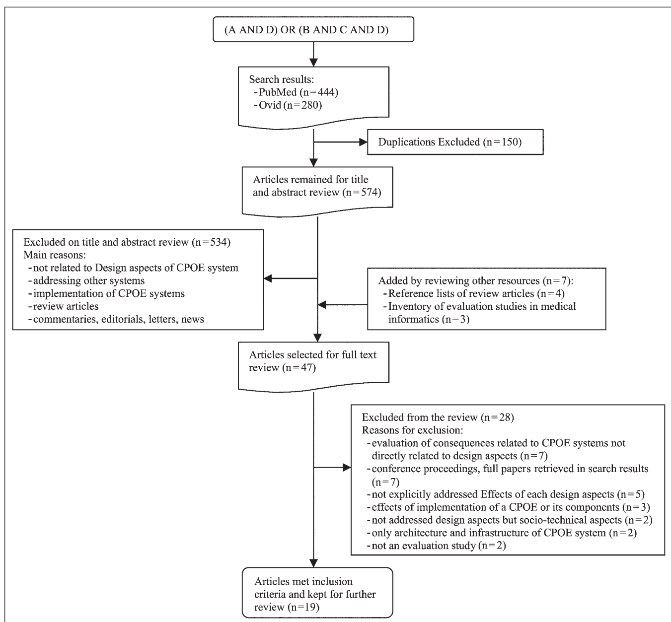
Fig. 2 Search flow
