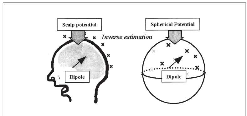
Fig. 1 The concept of the inverse estimation of dipoles.
