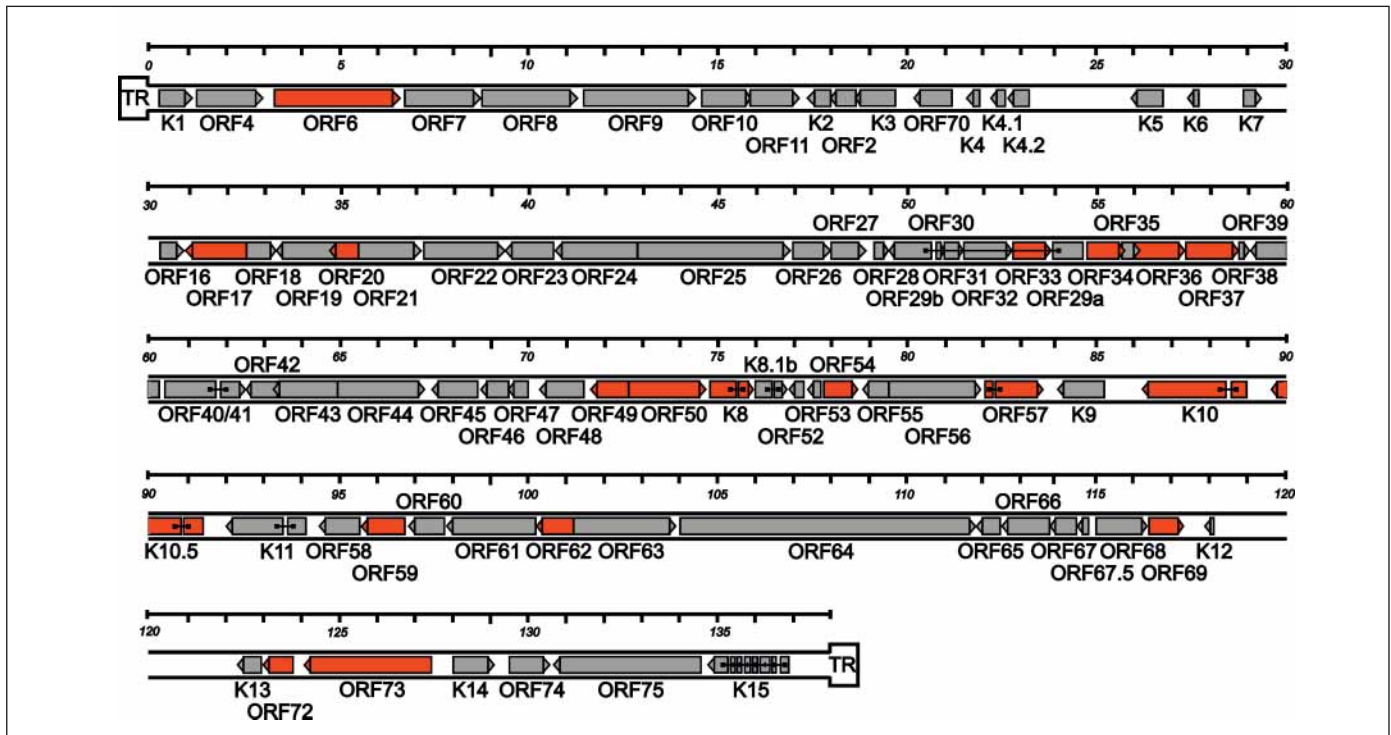
Figure 1: Gene map and nuclear localisation of KSHV proteins. Protein coding regions are indicated by arrows, and gene names are given (orfs: homologous to herpesvirus saimiri; K-genes: unique at time of sequencing). Orientations of the arrows indicate transcriptional orientations. Genes encoding proteins with exclusively nuclear localisation are labelled in red. Figure adopted with modifications from (86).
