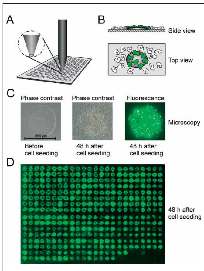
Figure 2: Reversely transfected cell array to determine signaling activity of over-expressed KSHV proteins.
