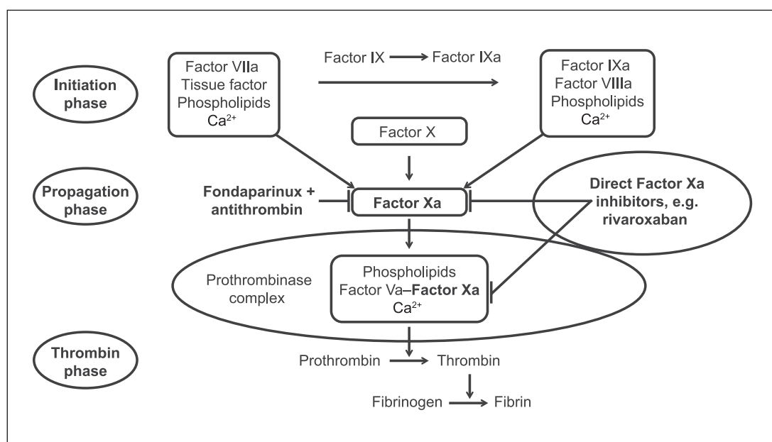
Figure 1: Different models of action of indirect factor Xa inhibitors (e.g. fondaparinux) and direct factor Xa inhibitors (e.g. rivaroxaban).
