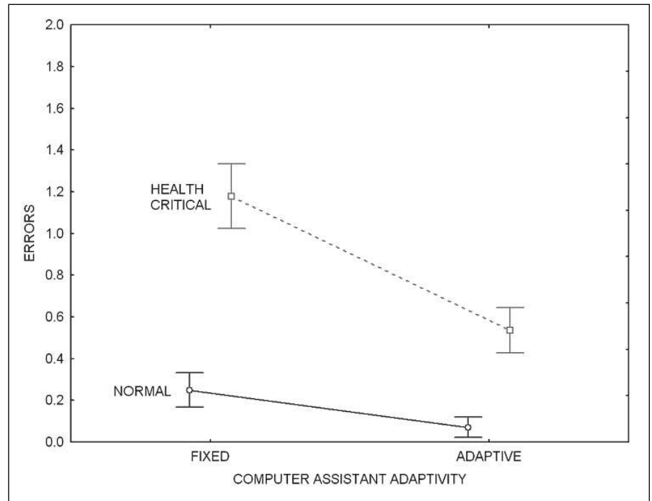
Fig. 3 Mean number of errors, with standard error bars, made in normal and health-critical situations with a fixed and adaptive computer assistant
